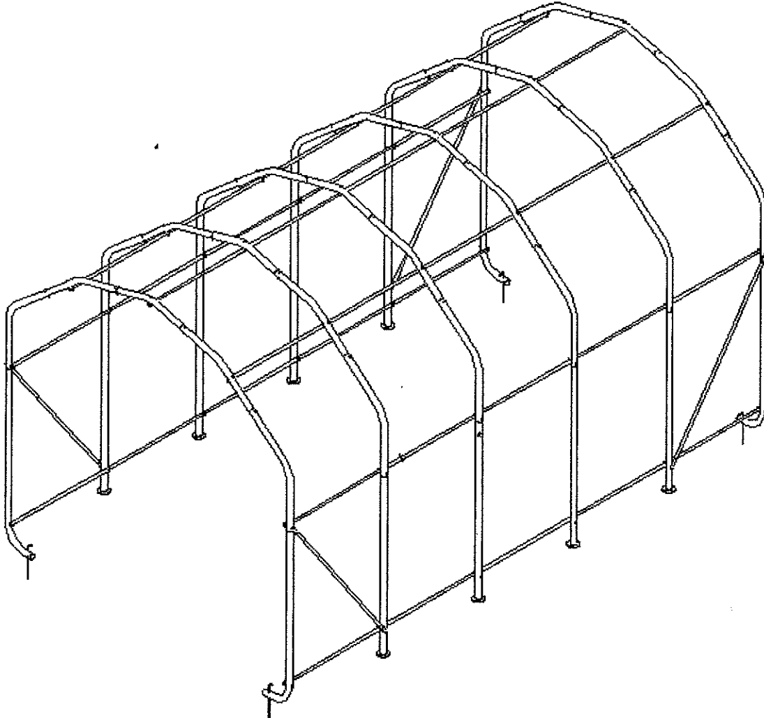
Barn Frame Assembly 12 x 20 x 10
