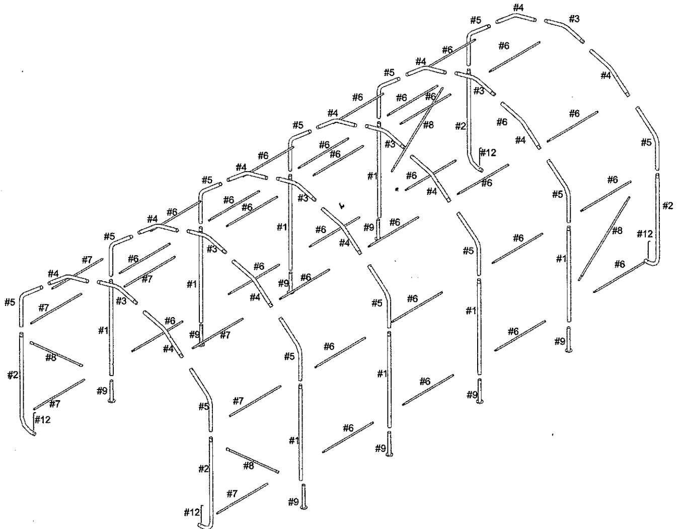
Frame Illustration Identified by Part Numbers 12 x 20 x 10 Barn Style
