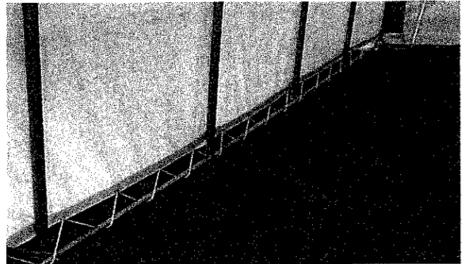
Lace rope through grommets and around Base Cross Rails
